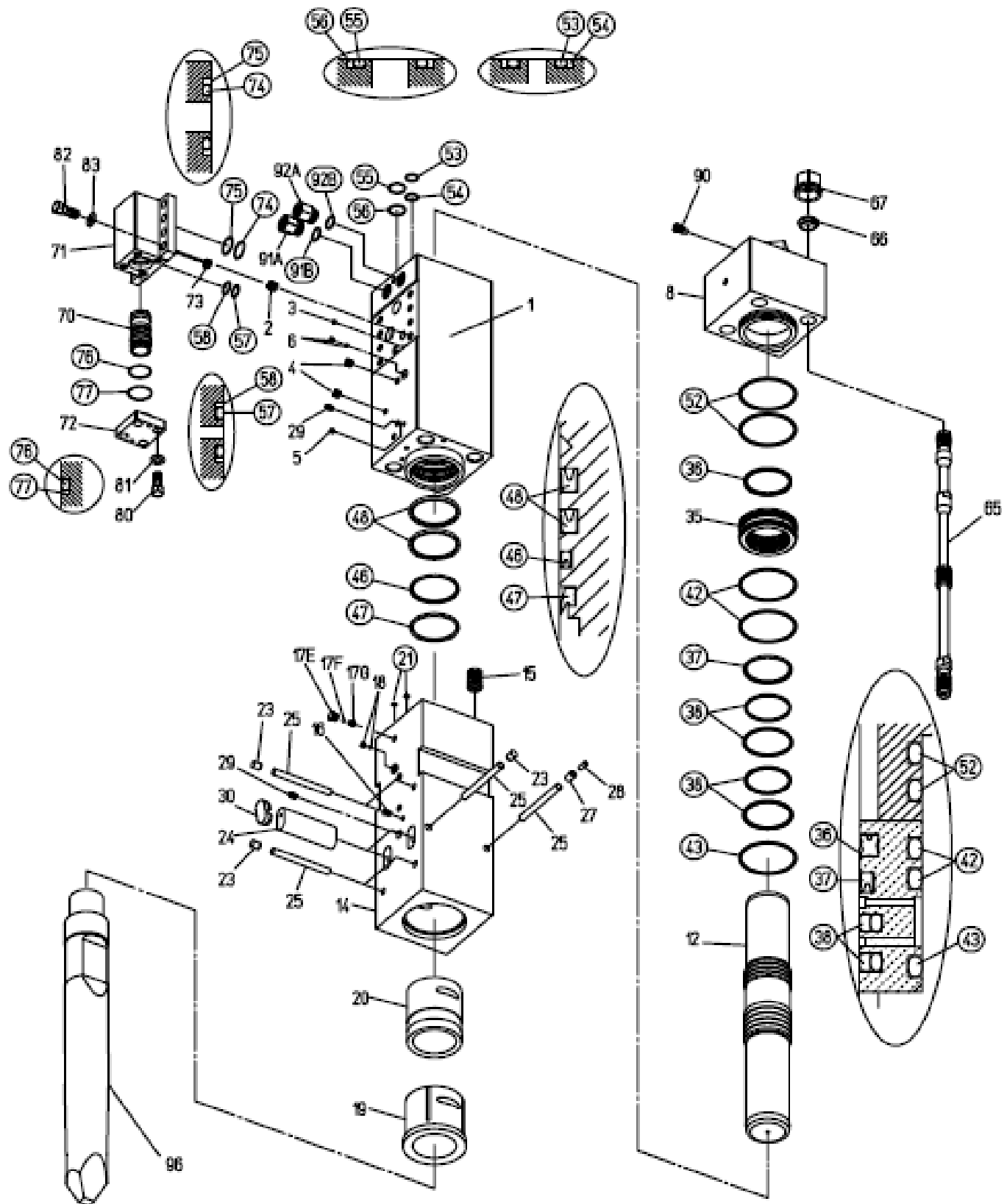
Parts & Price List for TNB-310LU 1 Hydraulic Breaker
